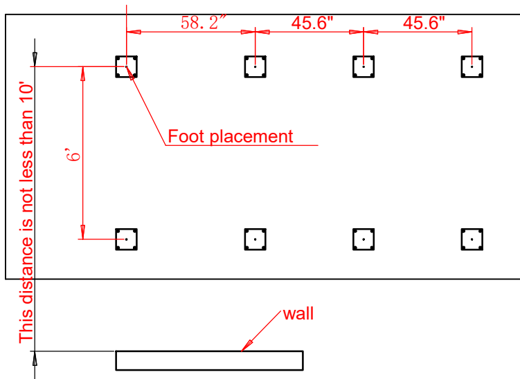
Foundation drawing
