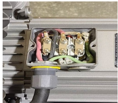
Figure 5-4: Vacuum Pump Wiring Example
