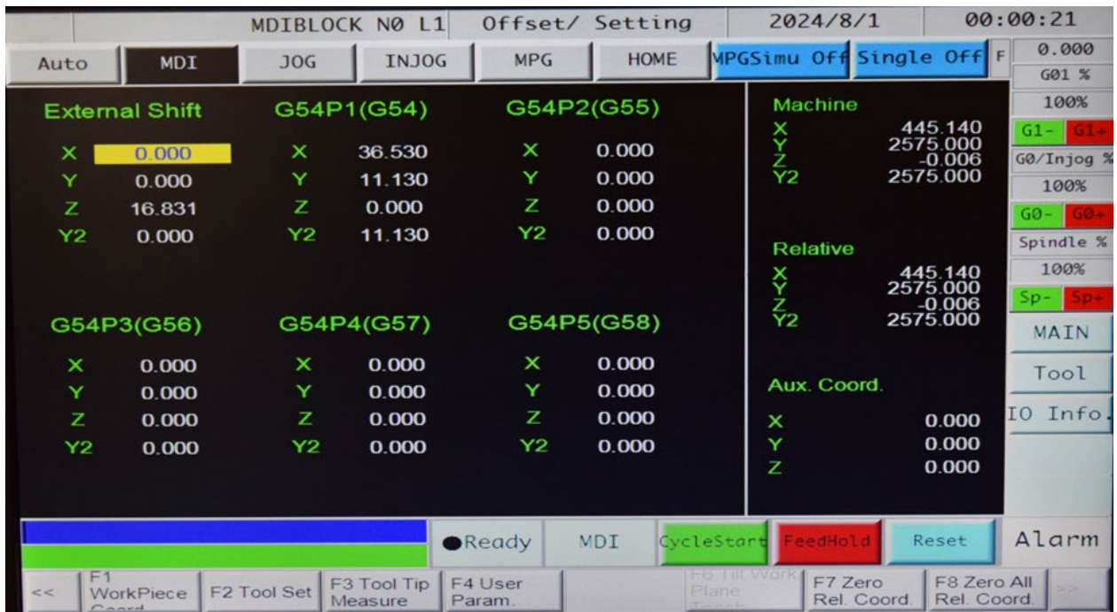
Figure 6-4: F3 Offset/Settings Screen
