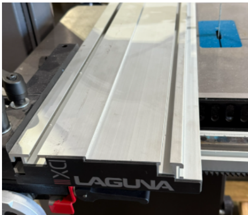
Fence in low position
